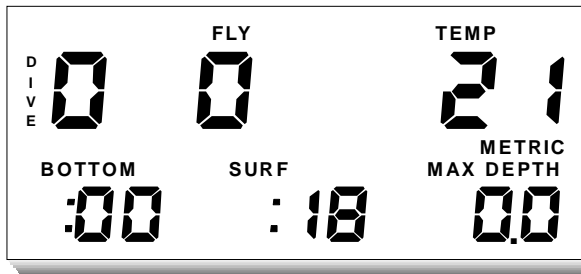
Figure 4 SURFACE MODE DISPLAY No Nitrogen Residual Dive of Day 0 Time to Fly 0 Temperature 21 c Bottom Time 0 Surface Time 18 mins MaxDepth 0 Altitude < 600 m tr Battery OK
