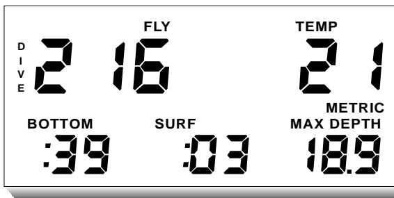
Figure 8 PO STD DIVE INTERVAL ("SURF" Legend Flashing)
