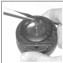
Fig. 47 - Retaining Ring
